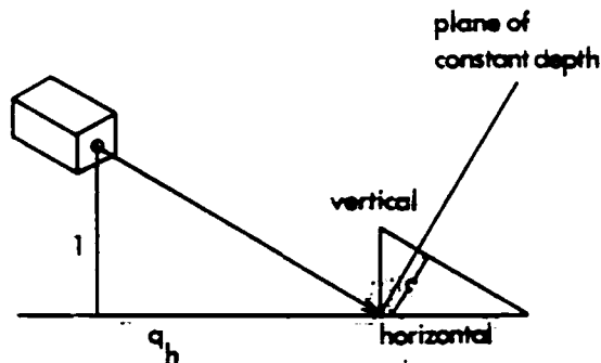
Figure 8-6: Right angle depths: side view.
