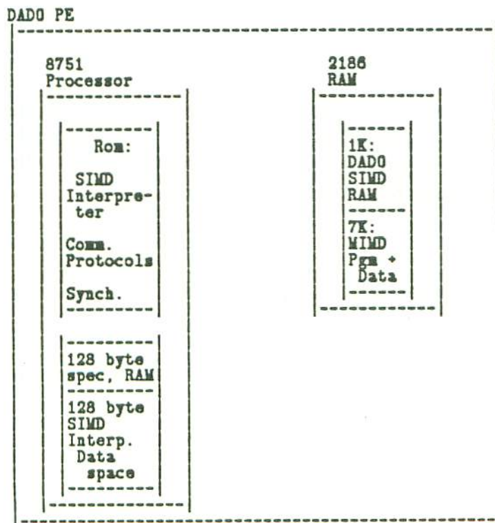
Figure 1: The DADO memory map
