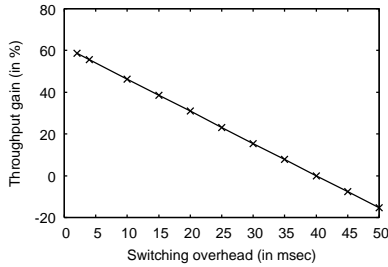
Figure 13: Impact of switching overhead on TCP throughput.
