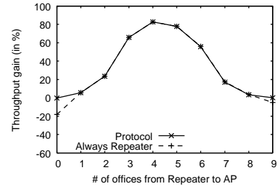
Figure 14: Max-min fairness: (a) Repeater Initiation Protocol is used, (b) SoftRepeater is always ON.
