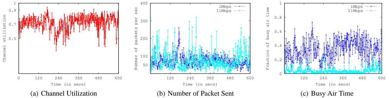
Figure 4: Analysis of the packets captured by a single sniffer on channel 1 during the Plenary Session of the 62 nd IETF.
