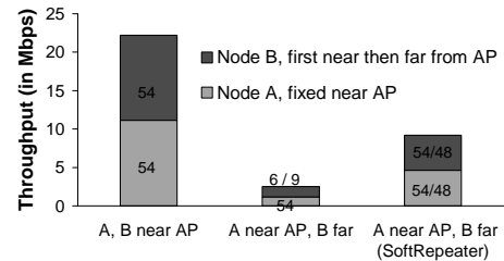
Figure 6: Downlink UDP flows, with and without SoftRepeater.
