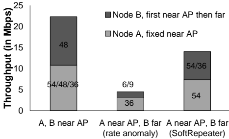
Figure 8: Uplink UDP flows, with and without SoftRepeater.
