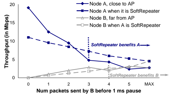
Figure 12: AP sends full blast traffic to A, and sends bursts of packets to B with a pause for 1 ms. MAX corresponds to back to back UDP packets.
