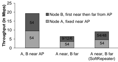
Figure 7: Downlink TCP flows, with and without a SoftRepeater.
