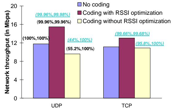
Figure 10: Throughput improvement due to network coding, and impact of RSSI optimization
