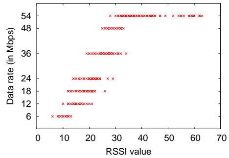
Figure 11: Correlation between RSSI and data rate.
