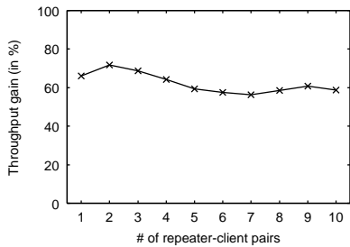
Figure 15: Improvement in throughput with multiple repeater-client pairs.
