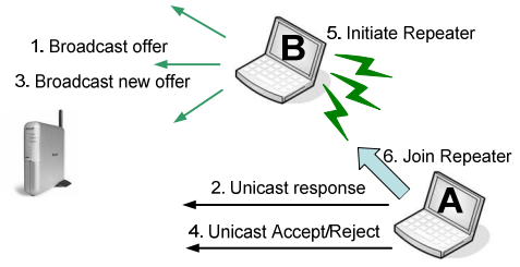
Figure 3: Steps of the Repeater Initiation Protocol.
