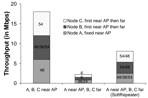
Figure 9: Downlink UDP flows when SoftRepeater serves two clients.
