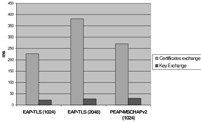
Fig. 9. Authentication delay in IEEE 802.11i
