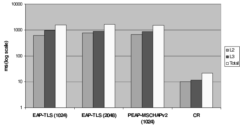
Fig. 10. Handoff time in IEEE 802.11i networks
