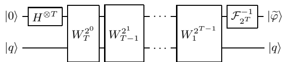
FIG. 1: The quantum phase estimation algorithm in power query notation. H is the Hadamard gate, W_l^p a power query as in equation (2), and \mathcal{F}_{2^T}^{-1} is the inverse quantum Fourier transform on T qubits.
