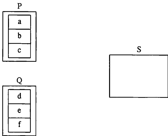
Figure 1: Communicating processes
