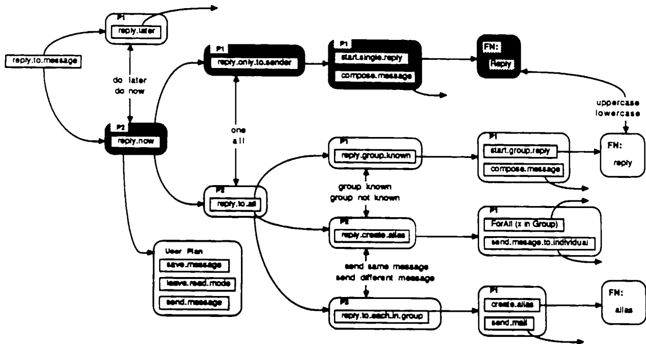
Figure 4-1: GENIE's Expert Model Knowledge of Replying to a Message
