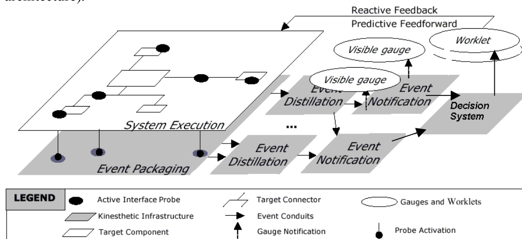
Figure 1: KX meta-architecture.
