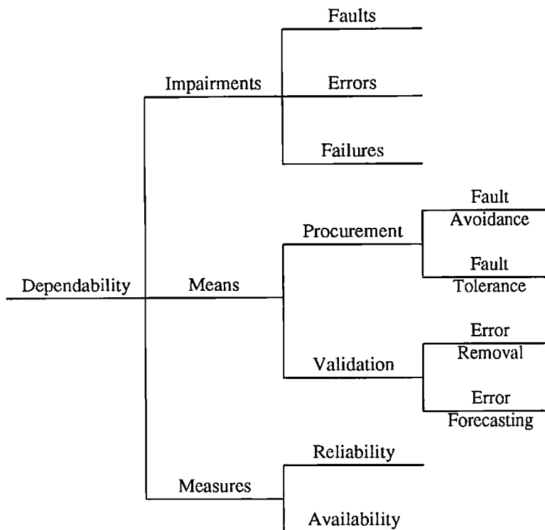
Figure 3: Laprie's Taxonomy
