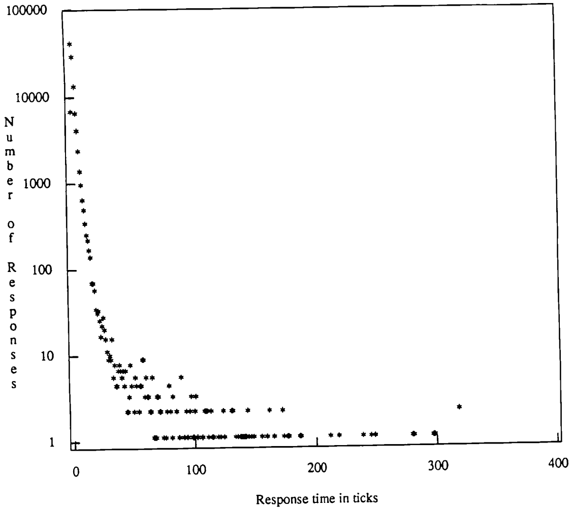
Number of Responses vs. Response time
