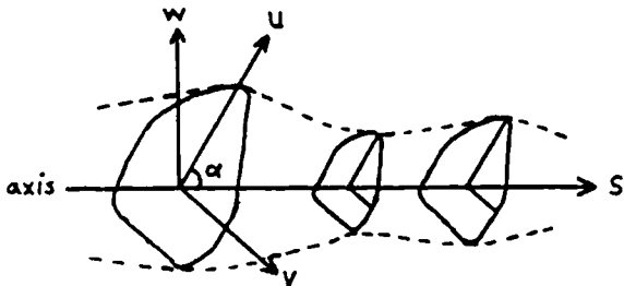
Figure 1: Straight Homogeneous Generalized Cylinder
