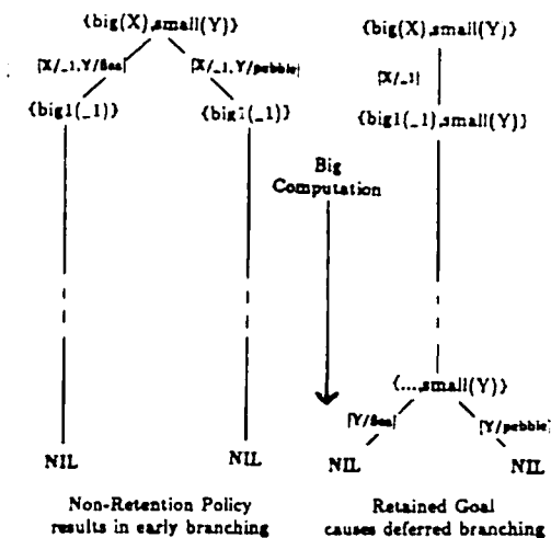
Figure 6-1: Goal retention postpones branching and may result in considerable savings of effort in the big - small problem
