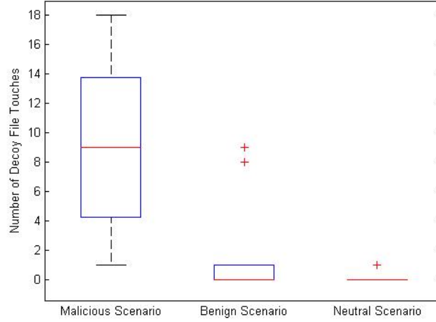
Fig. 6. Distribution of the Number of Decoy Document Accesses by Scenario
