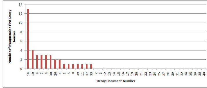
Fig. 8. Decoy File First Touches
