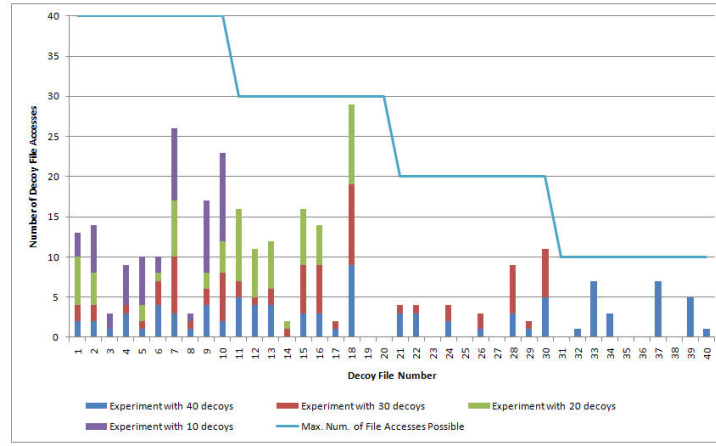
Fig. 9. Number of Decoy Document Accesses
