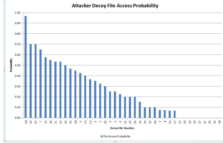
Fig. 10. Probability of an Attacker Opening the Decoy File
