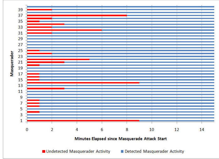
Fig. 7. Detection Time by User
