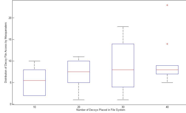
Fig. 5. Distribution of the Number of Decoy Document Accesses
